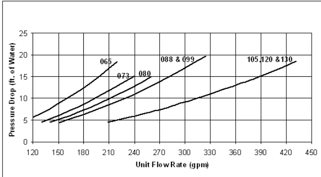
Figure 39: Mechanical Cooling Only
