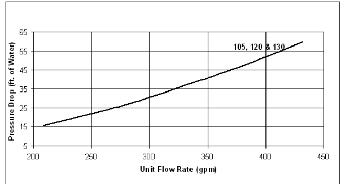
Figure 42: Large Economizer Coil
