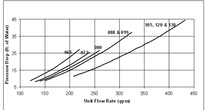
Figure 41: Mechanical Cooling and WRV
