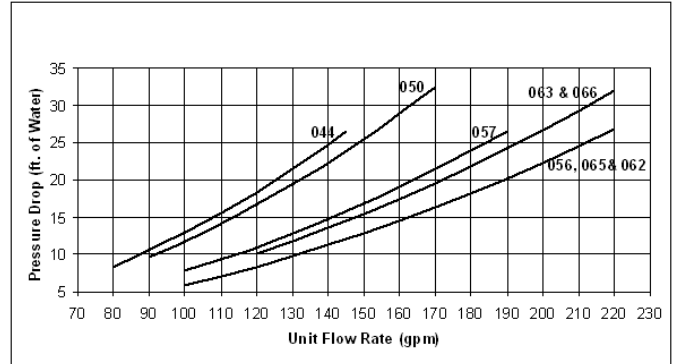
Figure 35: Large Economizer Coil
