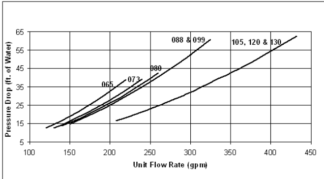
Figure 40: Standard Economizer Coil
