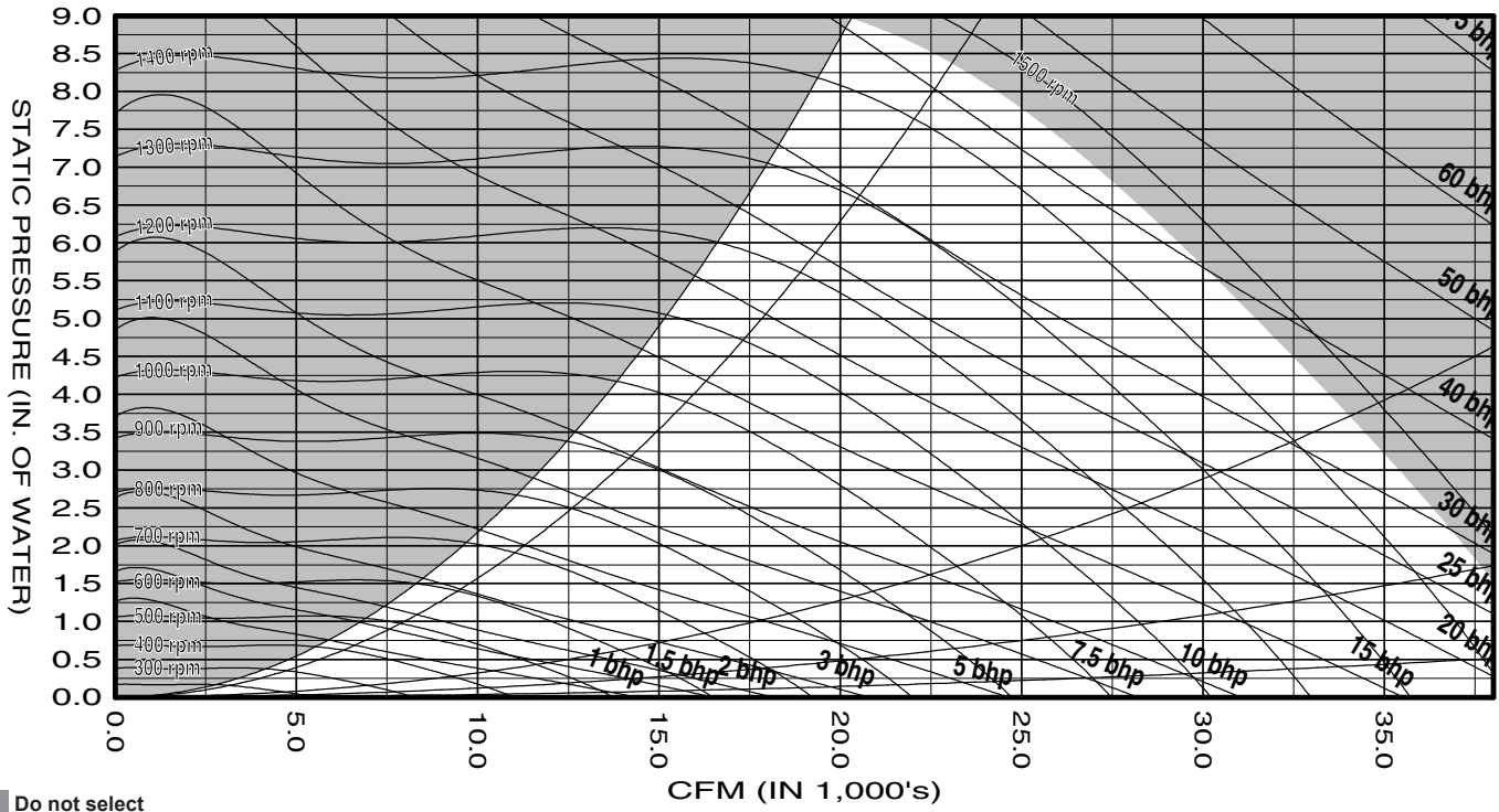
Figure 53: 36.5", 9-Blade Fan
