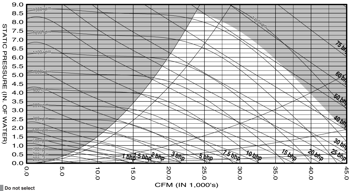
Figure 54: 40.2", 9-Blade Fan
