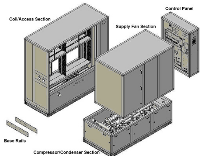
Figure 3: SWP Modular Sections
