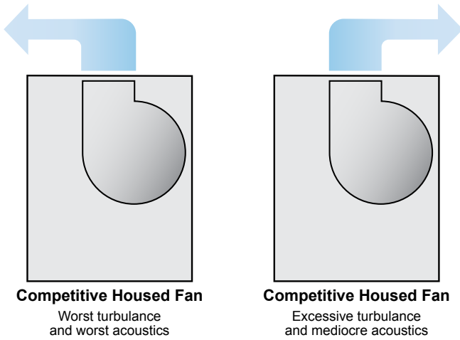
Figure 9: Supply Fan Comparison
