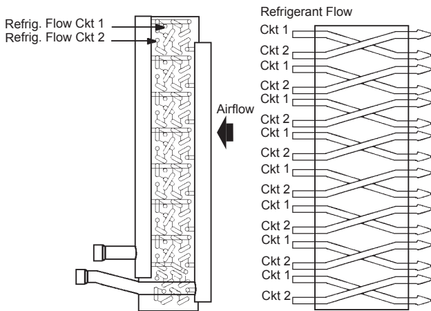
Figure 6: Evaporator Coil Circuiting
