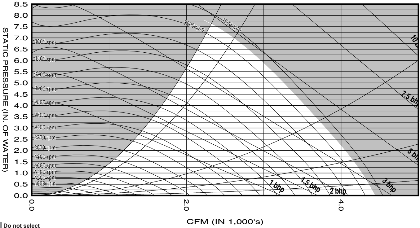
Figure 43: 13.5" Diameter, 9-Blade Fan
