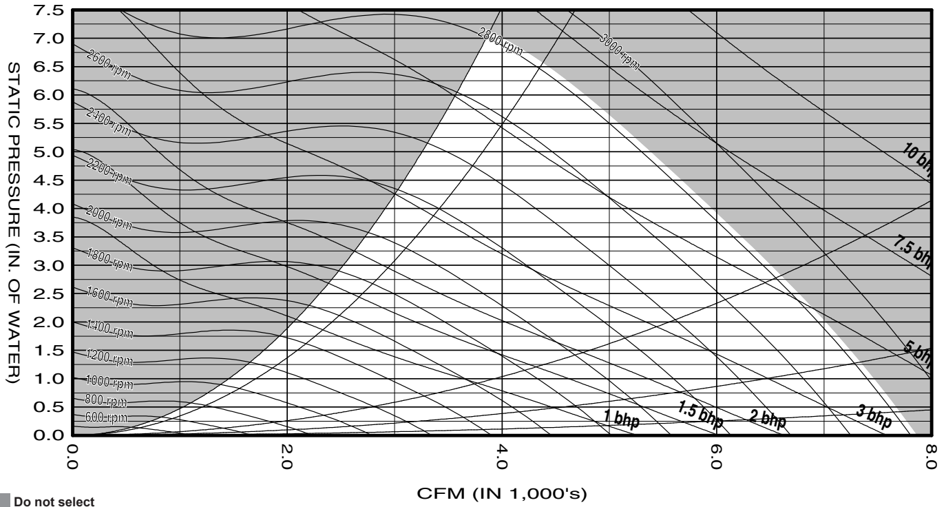
Figure 45: 16.5", 9-Blade Fan
