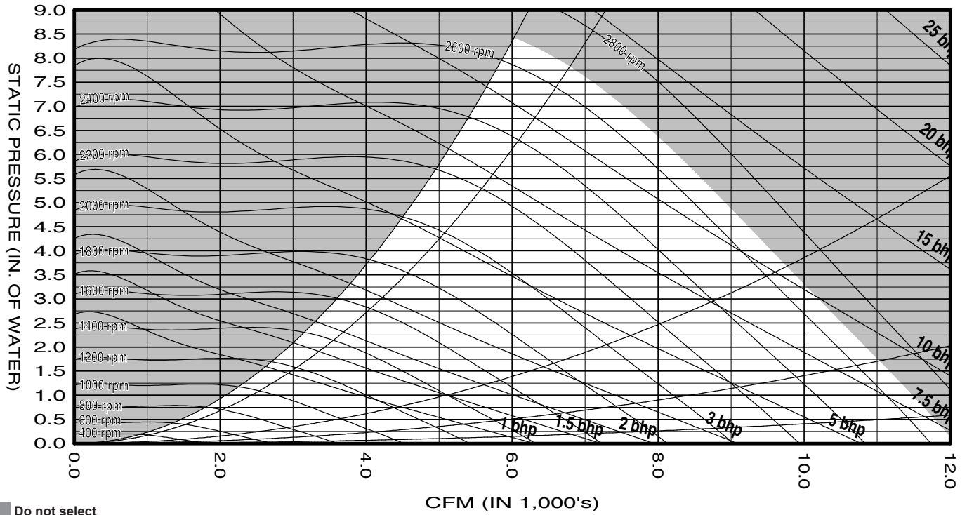
Figure 47: 20.0", 9-Blade Fan
