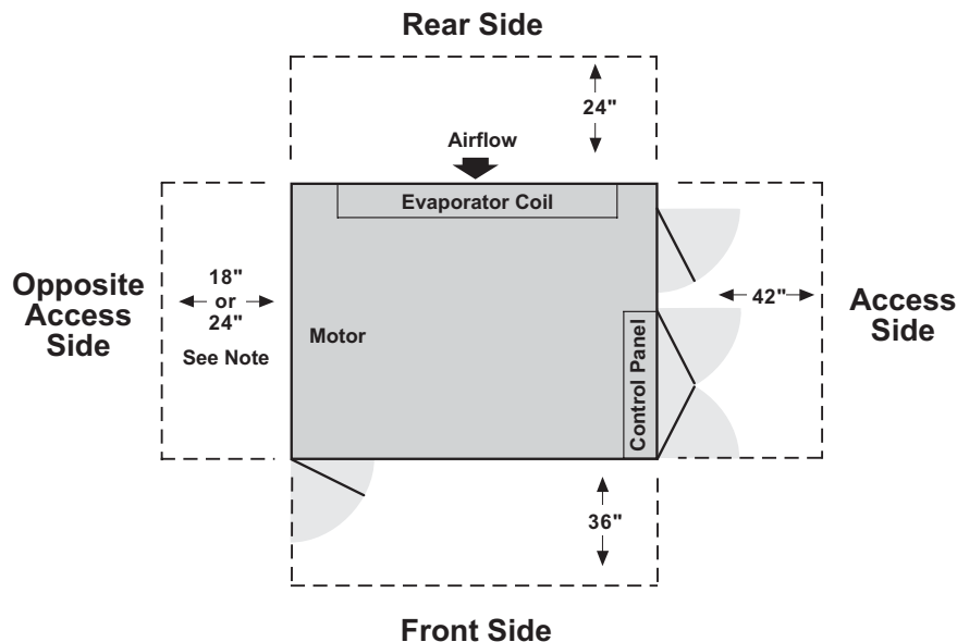
Figure 19: Recommended Service and Maintenance Clearances
