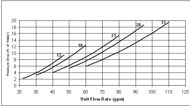
Figure 25: Standard Economizer Coil
