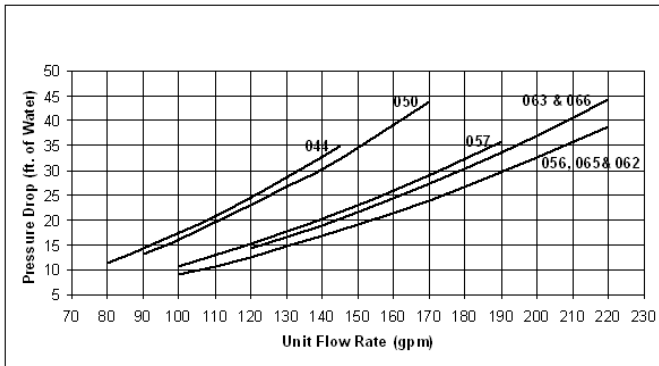
Figure 33: Standard Economizer Coil
