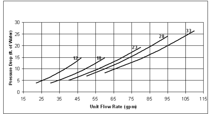
Figure 27: Large Economizer Coil
