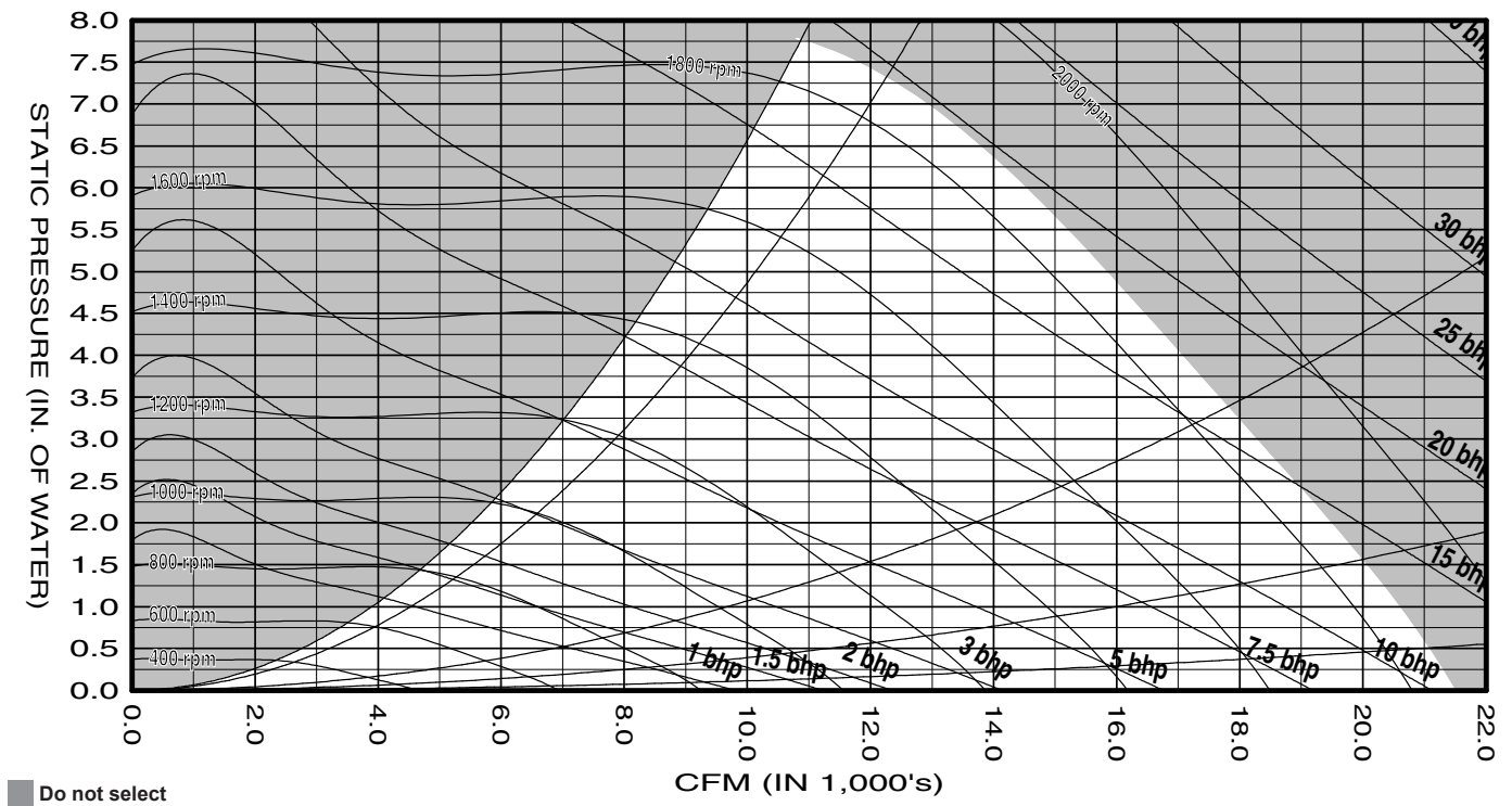
Figure 50: 27.0", 9-Blade Fan
