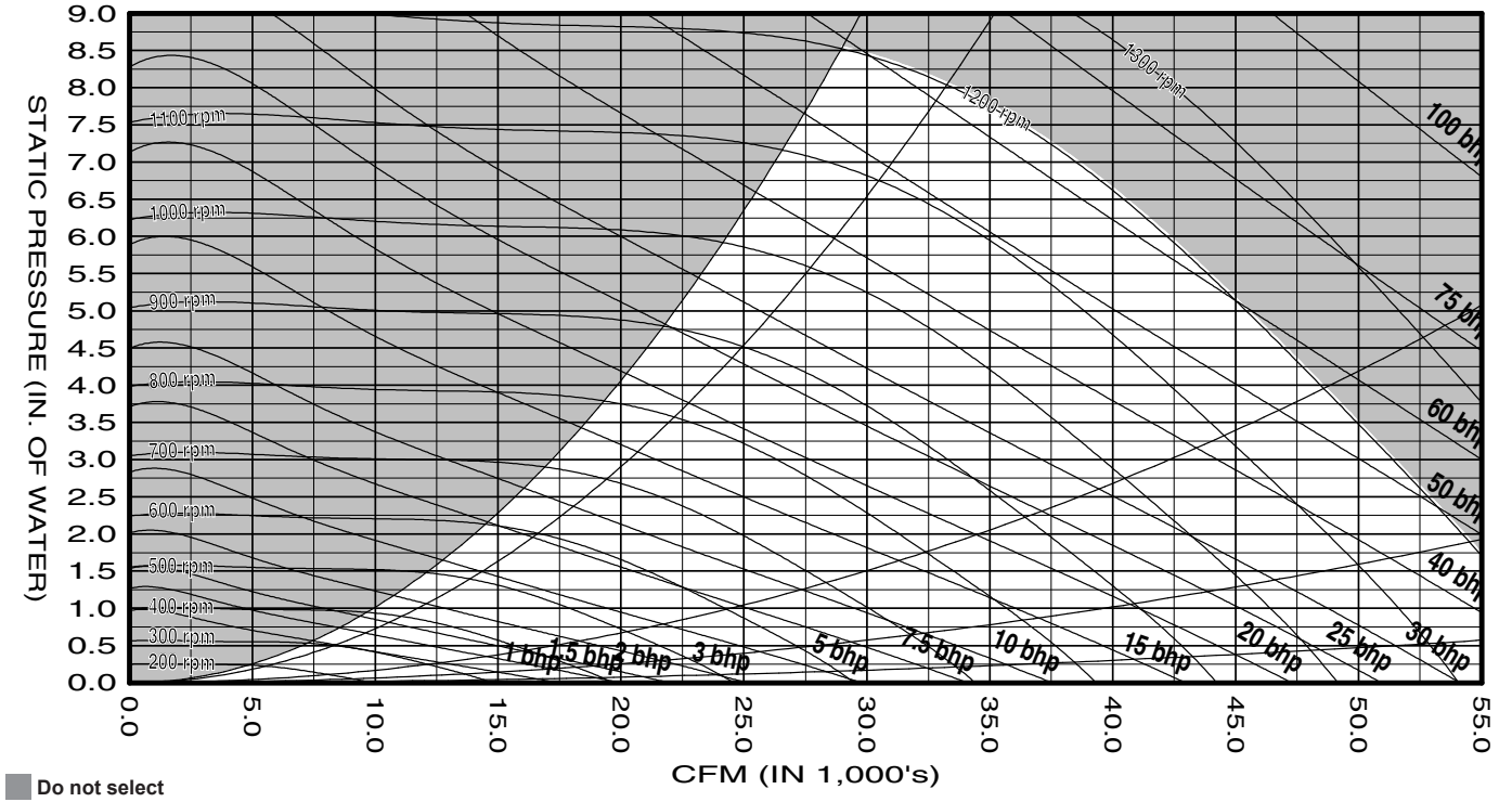
Figure 55: 44.5", 9-Blade Fan
