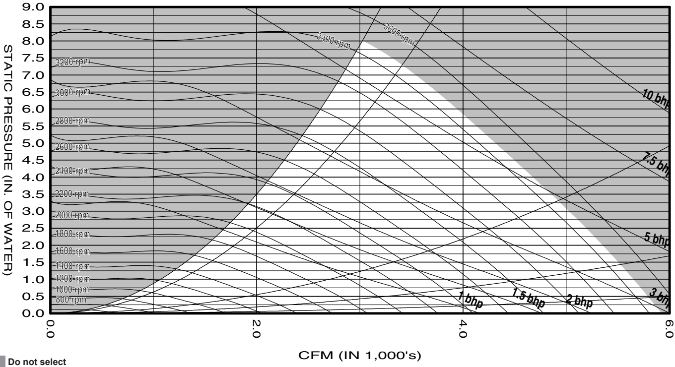
Figure 44: 15.0" Diameter, 9-Blade Fan
