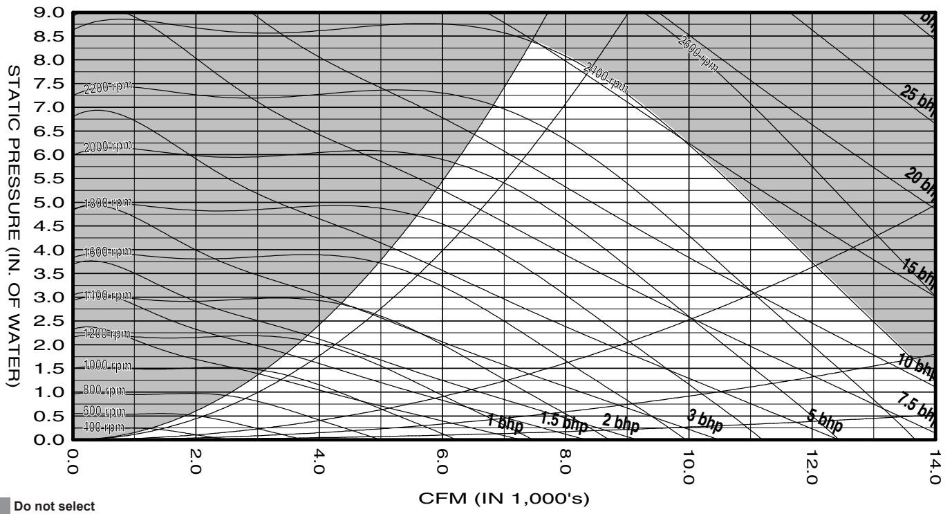
Figure 48: 22.2", 9-Blade Fan
