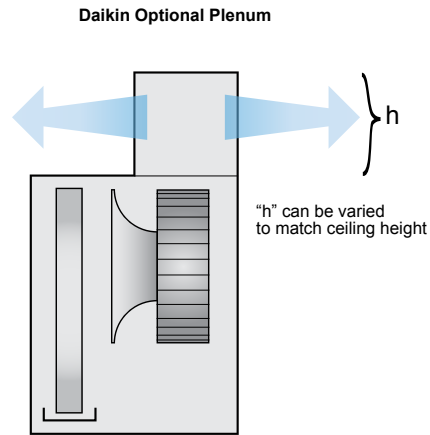
Figure 10: Acoustical Discharge Plenum
