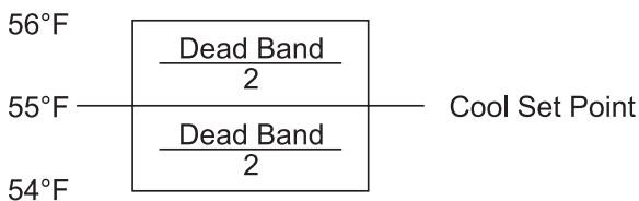
Figure 18: Compressorized Logic
