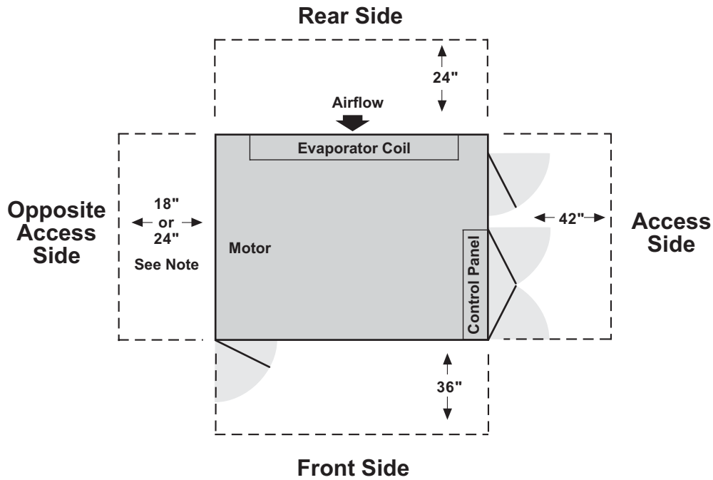
Figure 56: Recommended Service and Maintenance Clearances
