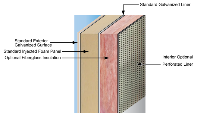
Figure 11: Foam Insulation and Sound Baffles
