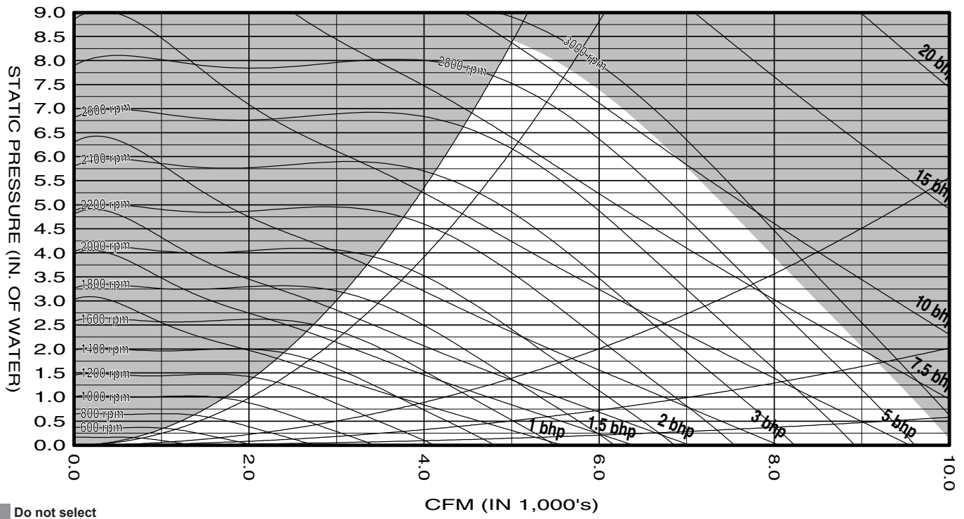
Figure 46: 18.2", 9-Blade Fan
