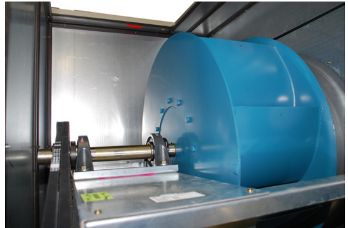
Figure 8: Airfoil Fan
