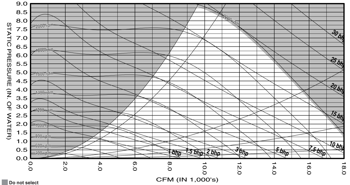
Figure 49: 24.5", 9-Blade Fan
