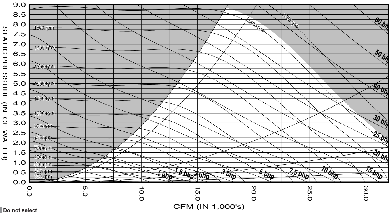
Figure 52: 33.0", 9-Blade Fan
