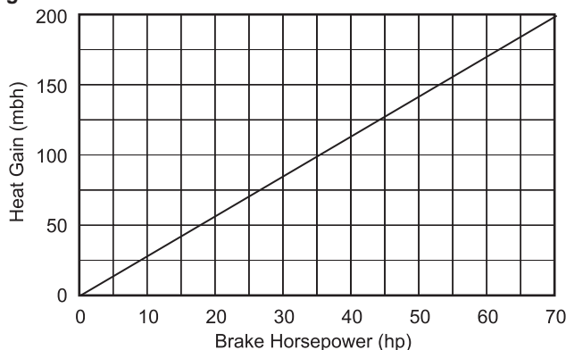
Figure 23: Fan and Motor Heat Gain
