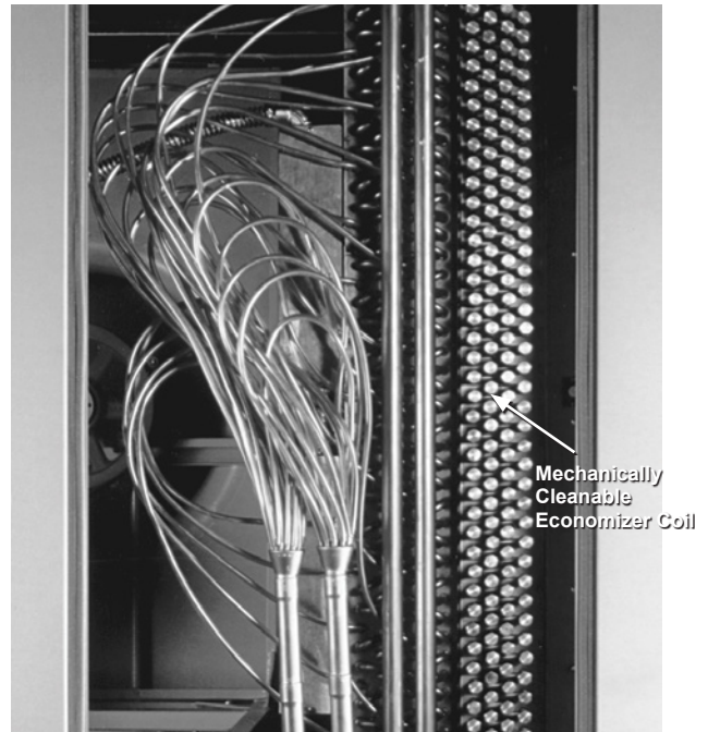
Figure 13: Mechanically Cleanable Waterside Economizer Coil
