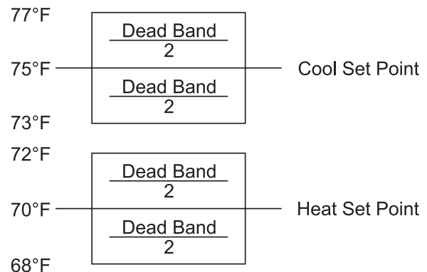
Figure 17: Control Temperature Logic
