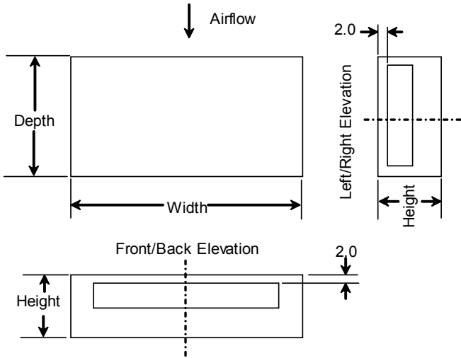
Figure 60: SWP Discharge Plenum Dimensions
