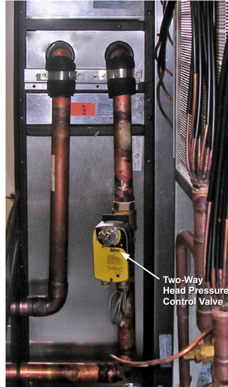
Figure 21: Head Pressure Control Valves
