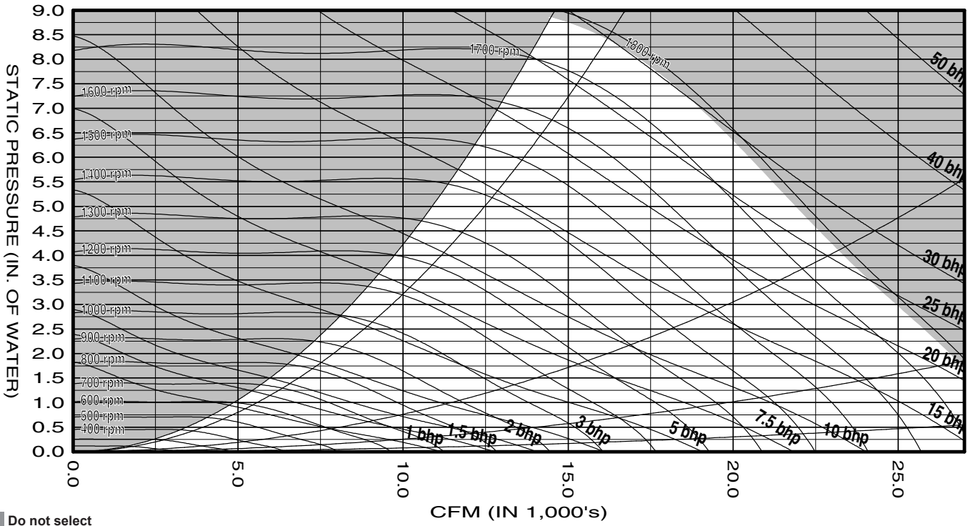
Figure 51: 30.0", 9-Blade Fan
