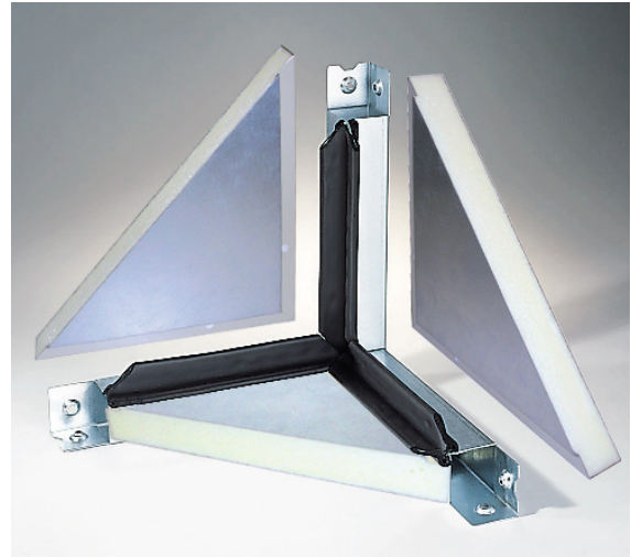
Figure 2: Hinged Access Doors with double latches
