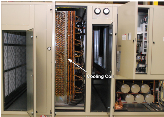
Figure 7: Cooling Coil Section Shown
