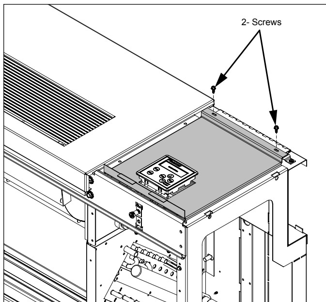
Figure 1: Install LUI into cutout in kit metal panel and secure panel with 2- screws
