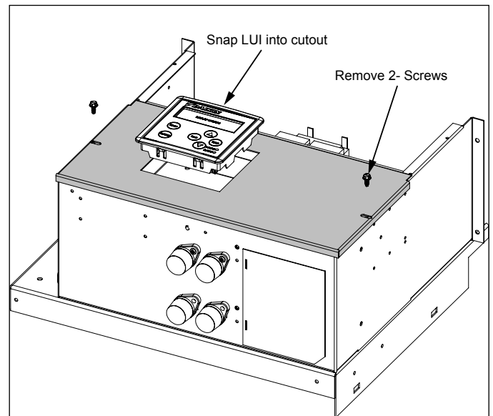
Figure 7: Install LUI into cutout in kit metal panel and secure panel with 2- screws
