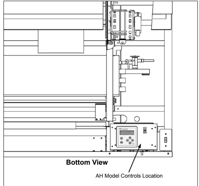
Figure 2: Location for LUI on AH unit
