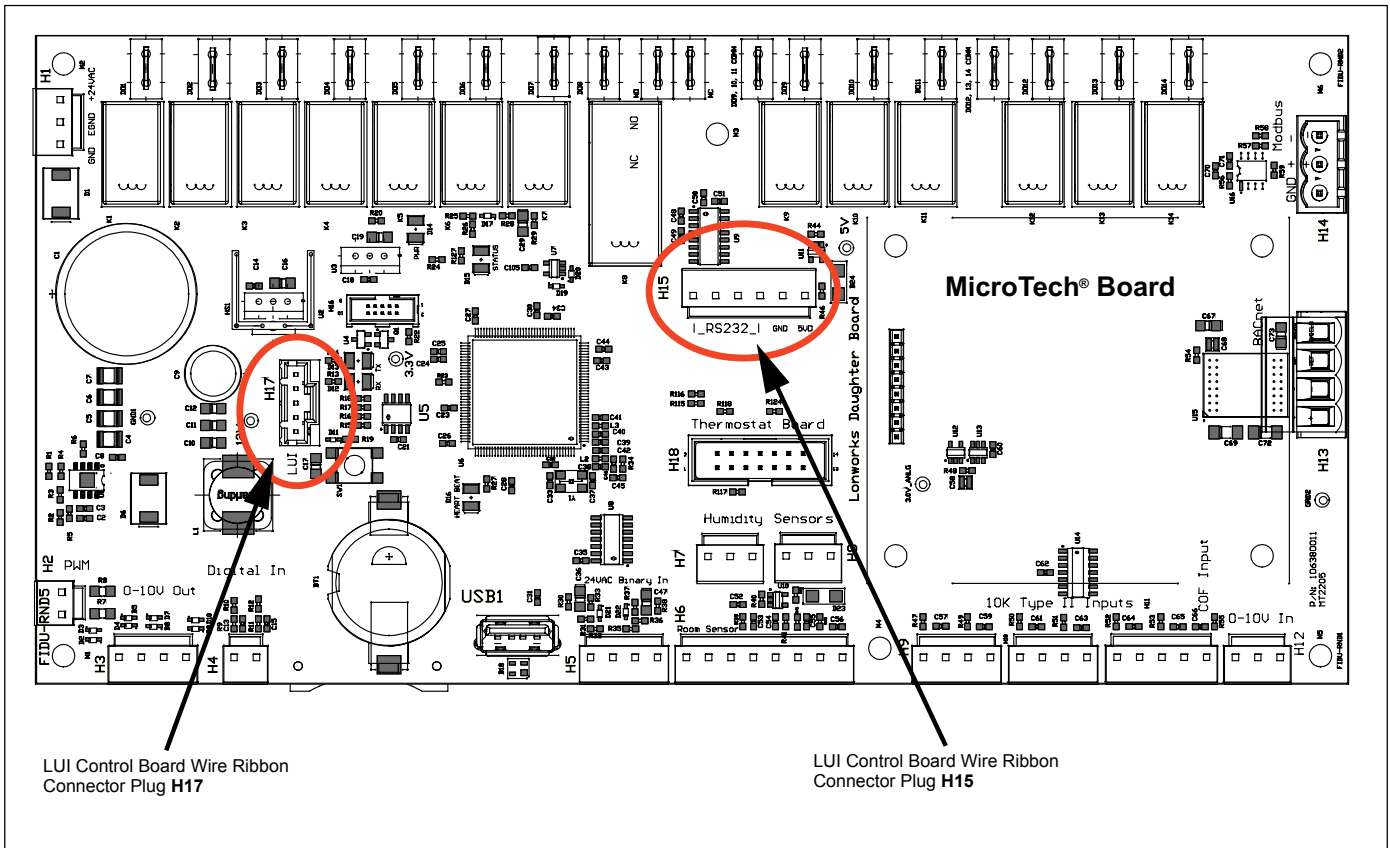
Figure 8: Control Board LUI Wire Ribbon Connections Locations – H15 & H17
