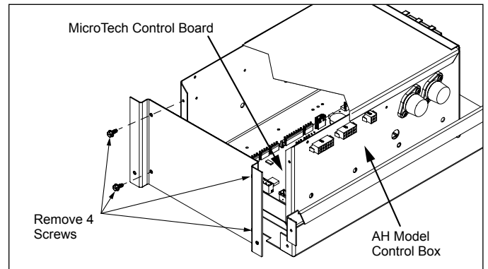
Figure 3: Remove the blank metal panel by removing 4- screws
