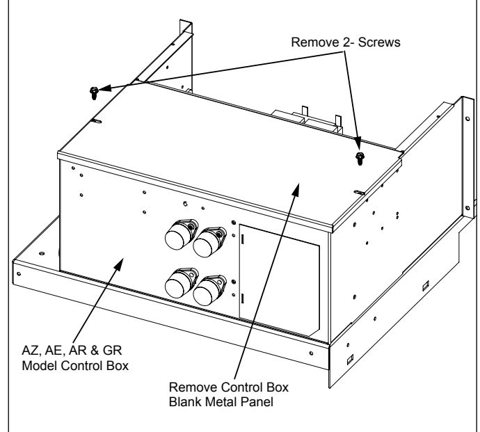
Figure 6: Remove control box blank metal panel
