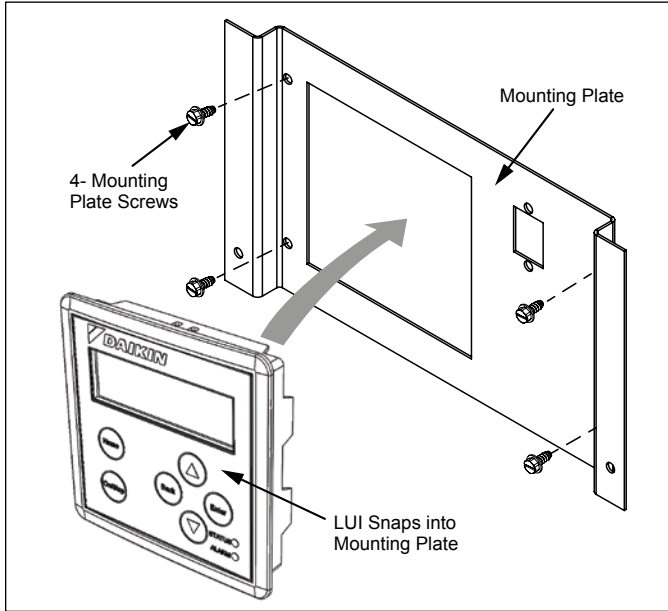
Figure 4: Snap LUI into cutout in kit metal panel
