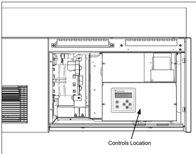
Figure 5: AZ, AE, AR & GR models control box location
