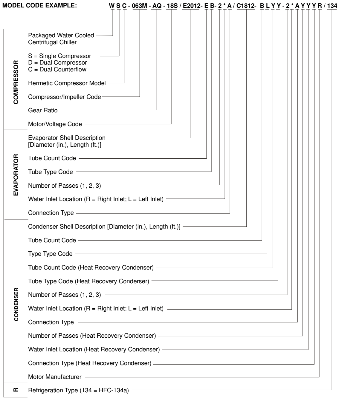
Figure 20, Chiller Identification
