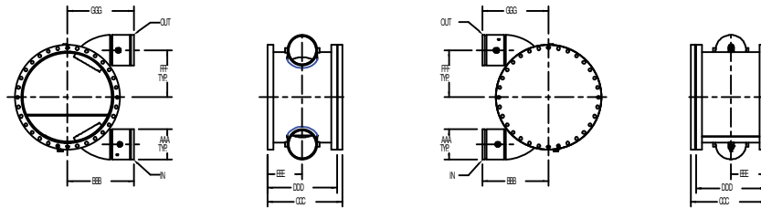
Dimensions with Victaulic or Flanged Connections (150 PSI Non-ASME - Victaulic Connection)
