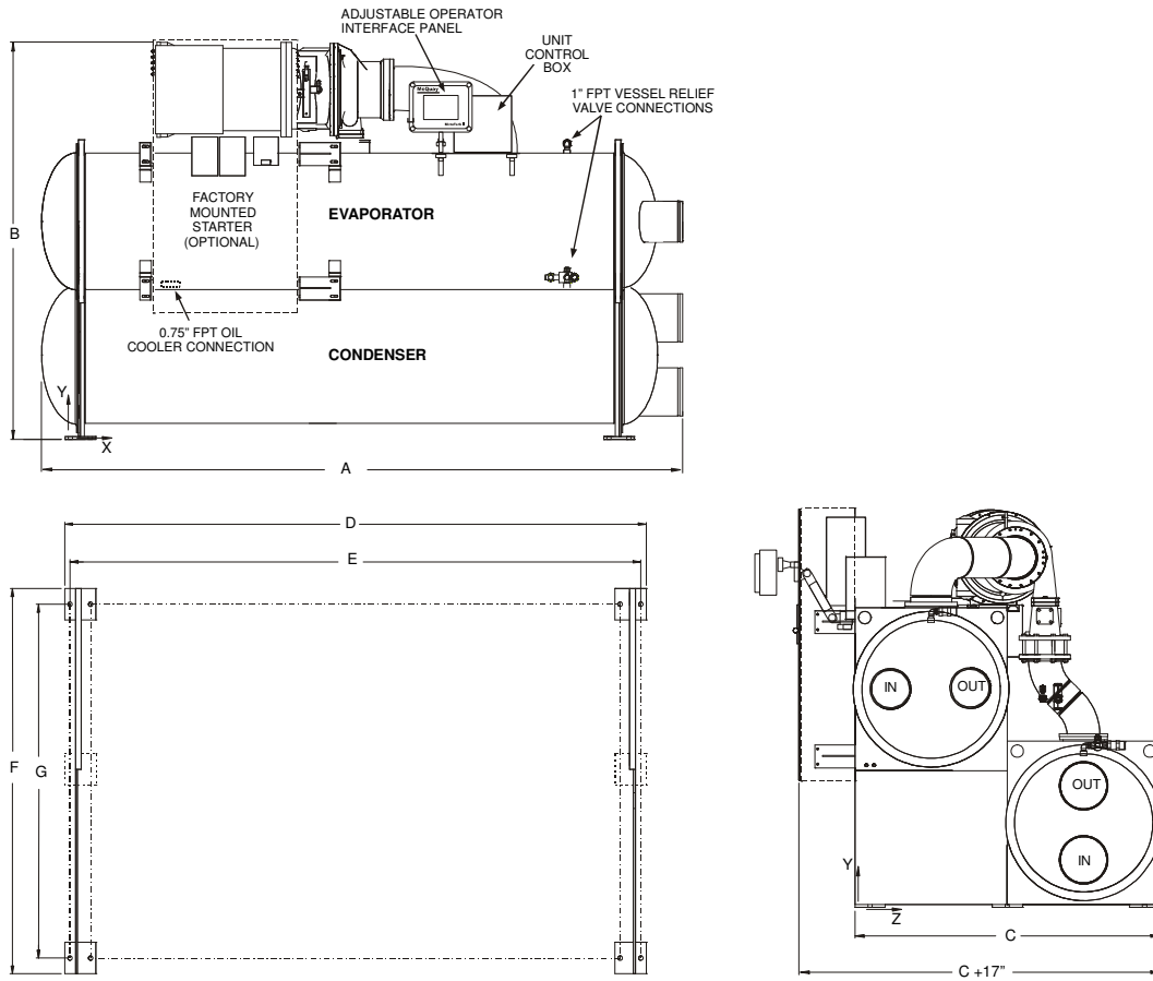
Figure 21, WSC 063, 160 to 300 Tons (560 to 1050 kW)
