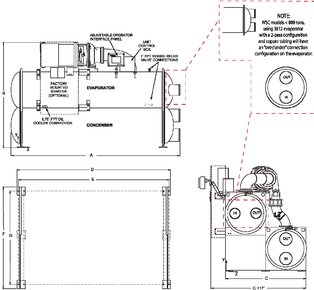
Figure 22, WSC 079/087, 300 to 600 Tons (1050 to 2110 kW)
