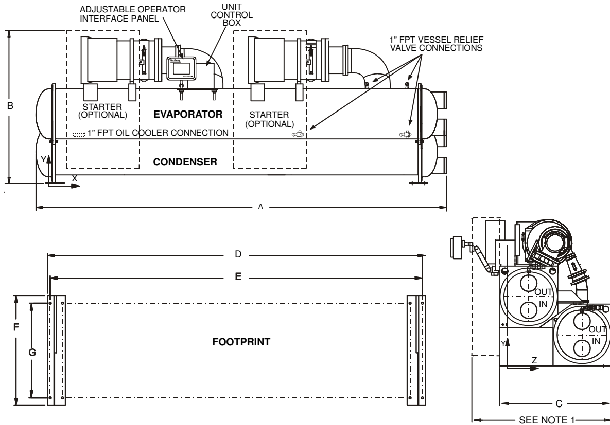
Figure 25, WDC 079 and WDC 087, 600 to 1200 tons (2100 to 4220 kW)
