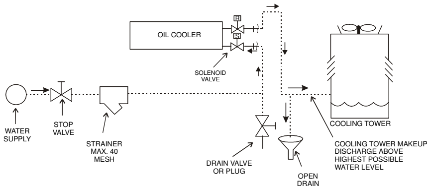
Figure 17, Oil Cooler Piping With City Water
