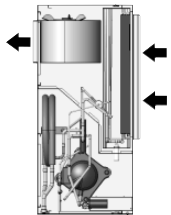
Figure 6D - Right Hand Return with Straight Discharge
