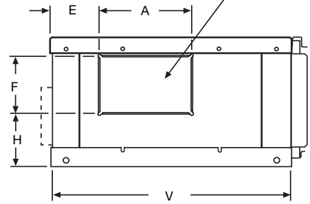
End Discharge View
